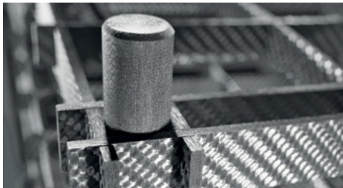
↑ Corner connection as C/C and graphite hybrid design
