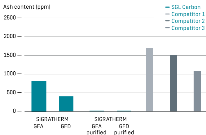
Comparison of purity of several soft felts via ash level analysis
