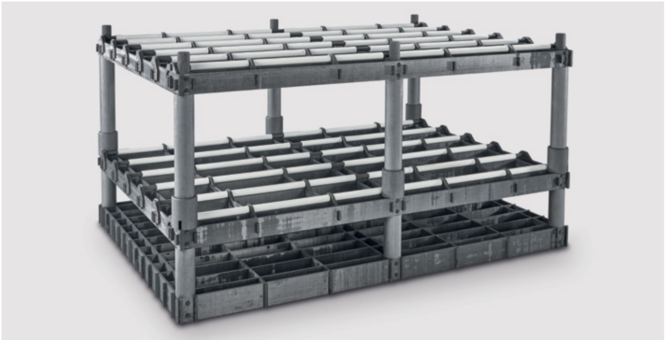
↑ SIGRABOND Performance C/C hybrid charging rack with ceramics for carburization protection
