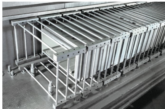
↑ Heating system of a continuous inert gas furnace designed with SIGRAFINE heating tubes and SIGRAFINE HLM muffle
