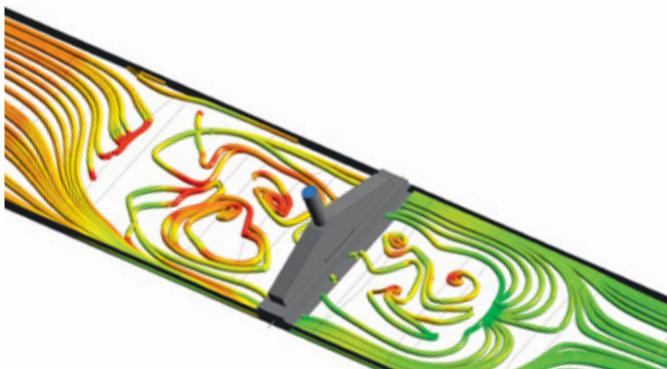
↑ FEM-CFD simulation of gas flow through a continuous high-temperature furnace
