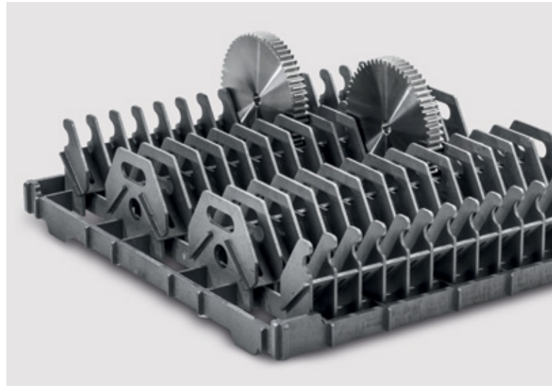
↑ Charging rack made from SIGRASIC Performance for heat treatment including preoxidation and oil quenching
